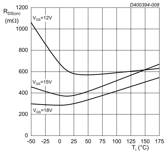
I_{DS} = 2\text{ A}; t_p < 200\text{ }\mu\text{s} Fig. 8. Drain-source on-state resistance as a function of junction temperature
